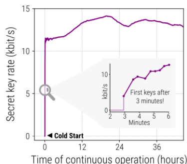
Figure 2: Continuous operation of the CV-QKD system with a key rate exceeding 10 kbit/s.
